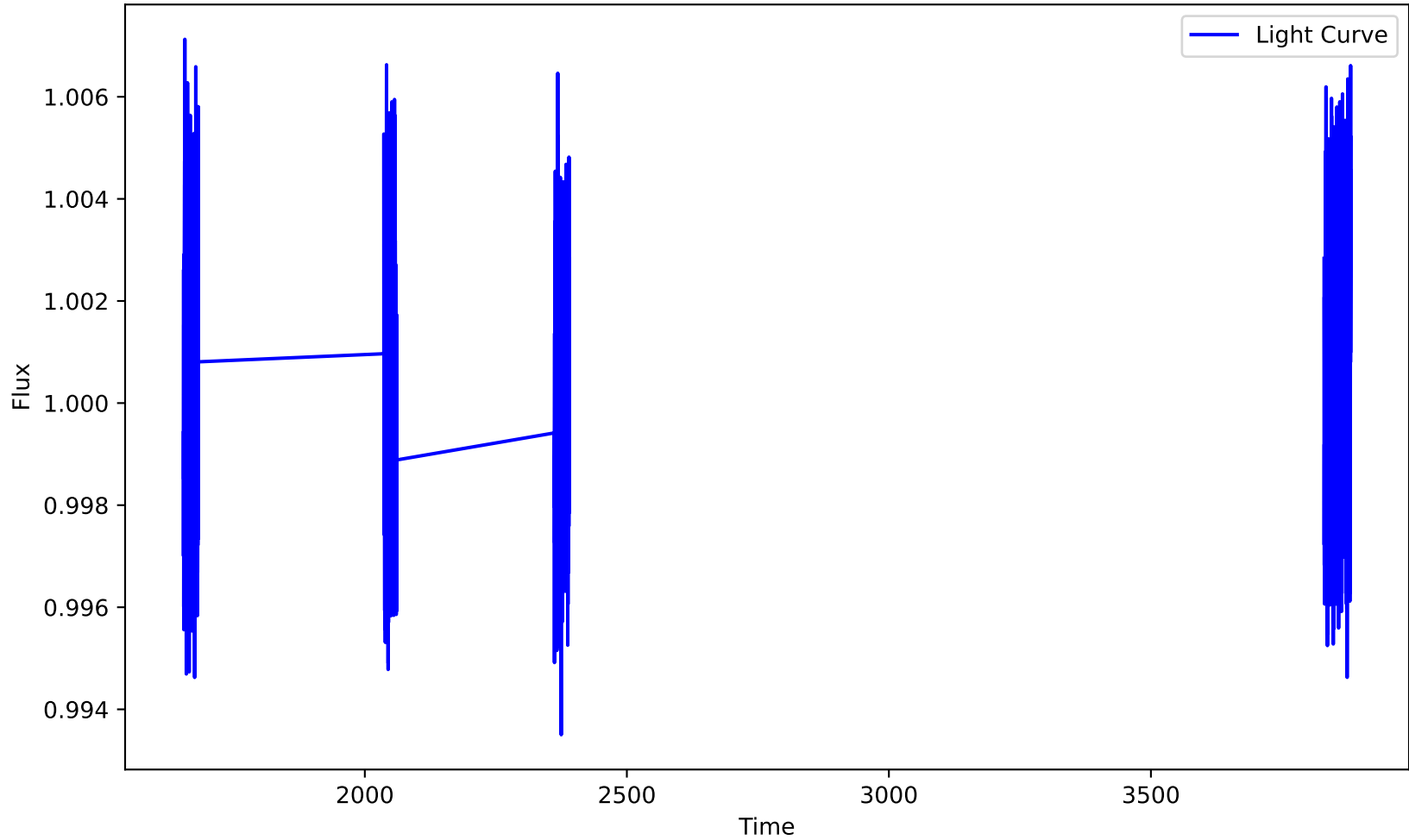
Light Curve
